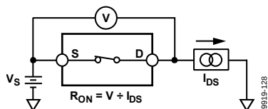
Figure 28. On Resistance
