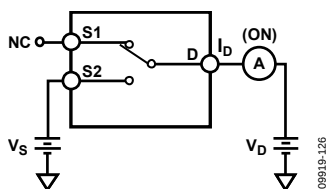
Figure 26. On Leakage
