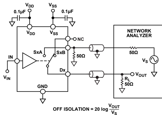
Figure 31. Off Isolation
