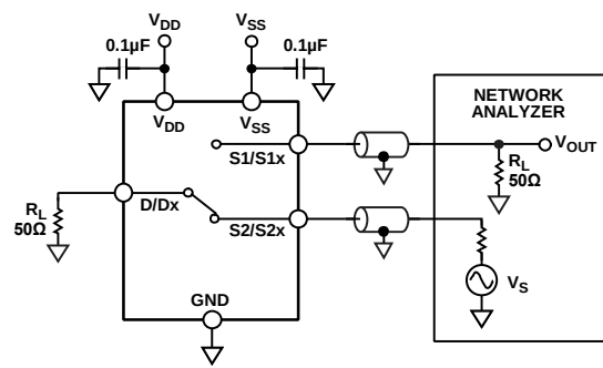
Figure 41. Bandwidth
