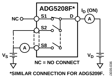
Figure 37. On Leakage
