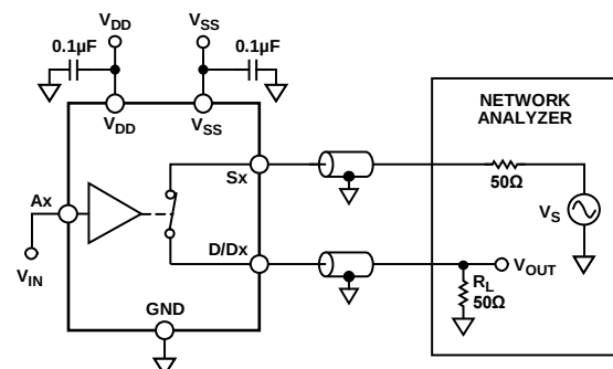
Figure 40. Off Isolation
