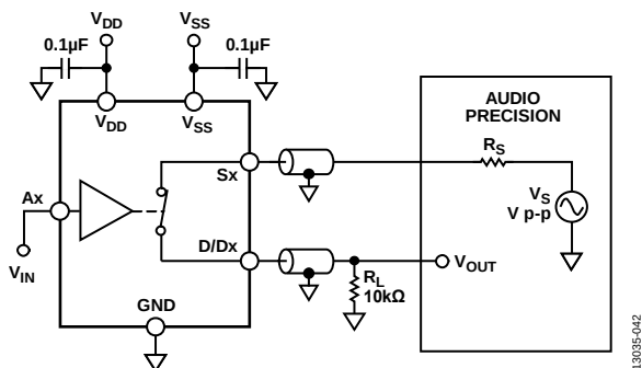
Figure 39. THD + N
