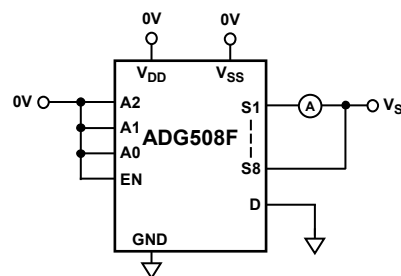
Figure 26. Input Leakage Current (with Power Supplies Off)
