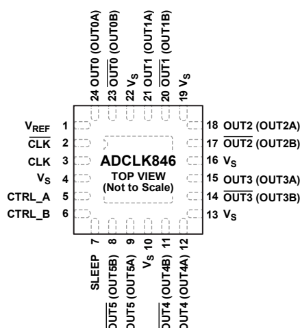
Figure 2. Pin Configuration
