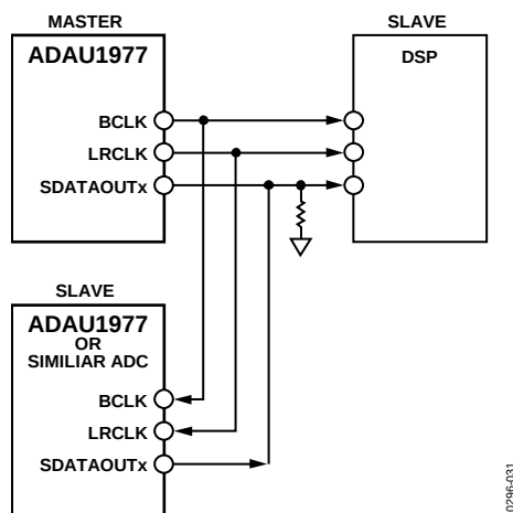
Figure 32. Serial Port Connection Option 3—TDM Mode, ADAU1977 Master
