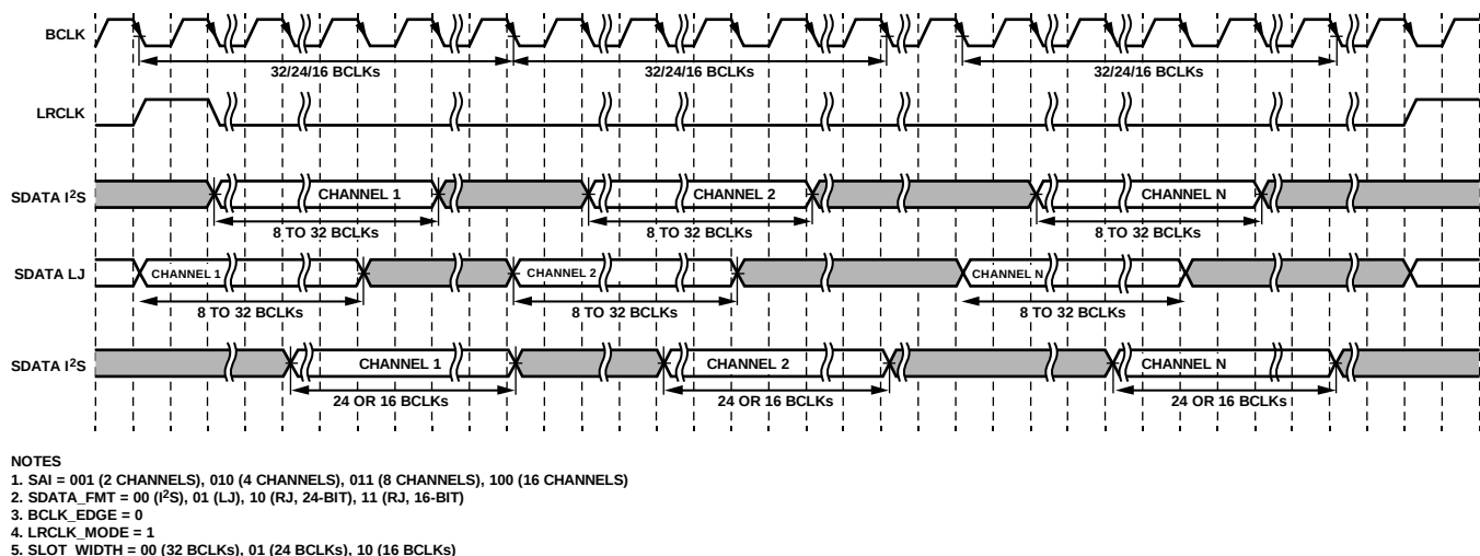
Figure 28. TDM Pulse Mode Audio Format
