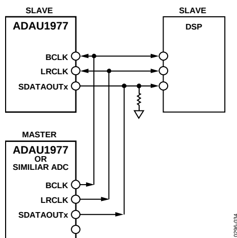
Figure 33. Serial Port Connection Option 4—TDM Mode, Second ADC Master
