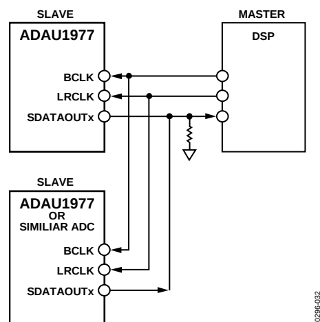
Figure 34. Serial Port Connection Option 5—TDM Mode, DSP Master
