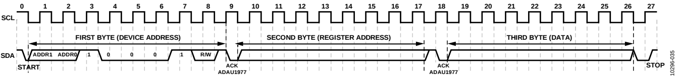
Figure 35. I 2 C Write to ADAU1977 Single Byte
