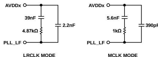
Figure 15. PLL Filter
