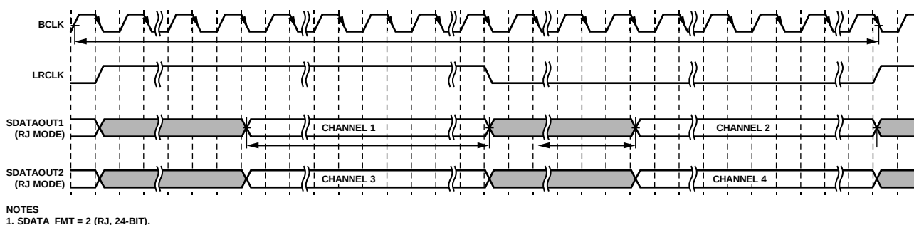
Figure 26. RJ Audio Format
