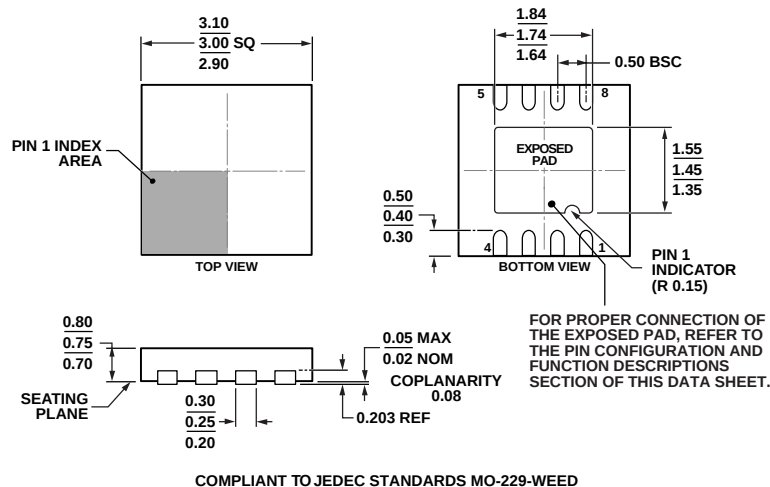
Figure 64. 8-Lead Lead Frame Chip Scale Package [LFCSP] 3 mm × 3 mm Body and 0.75 mm Package Height (CP-8-13) Dimensions shown in millimeters
