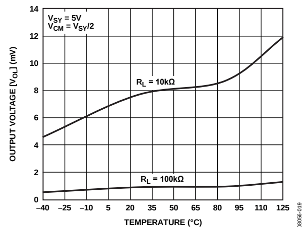
Figure 22. Output Voltage ( V_O ) vs. Temperature
