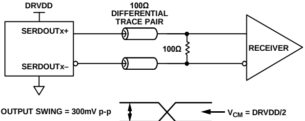
Figure 160. DC-Coupled Digital Output Termination Example
