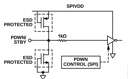
Figure 113. PDWN/STBY Input
