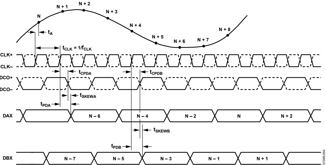
Figure 3. Interleaved Mode
