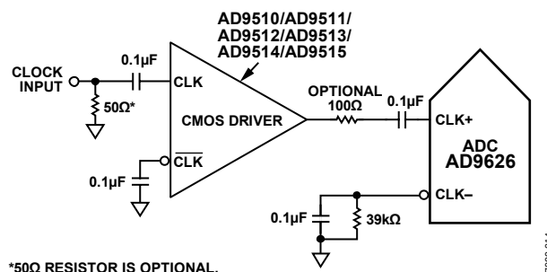
Figure 48. Single-Ended 1.8 V CMOS Sample Clock
