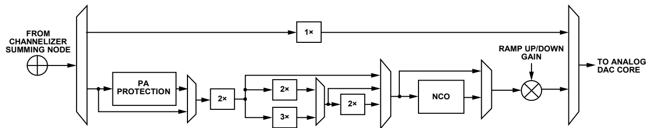
Figure 74. Block Diagram of the Main Digital Datapath per Main DAC Output
