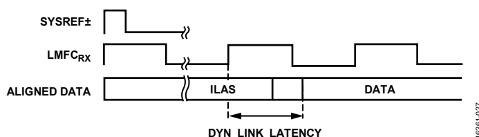
Figure 65. DYN_LINK_LATENCY_x Illustration
