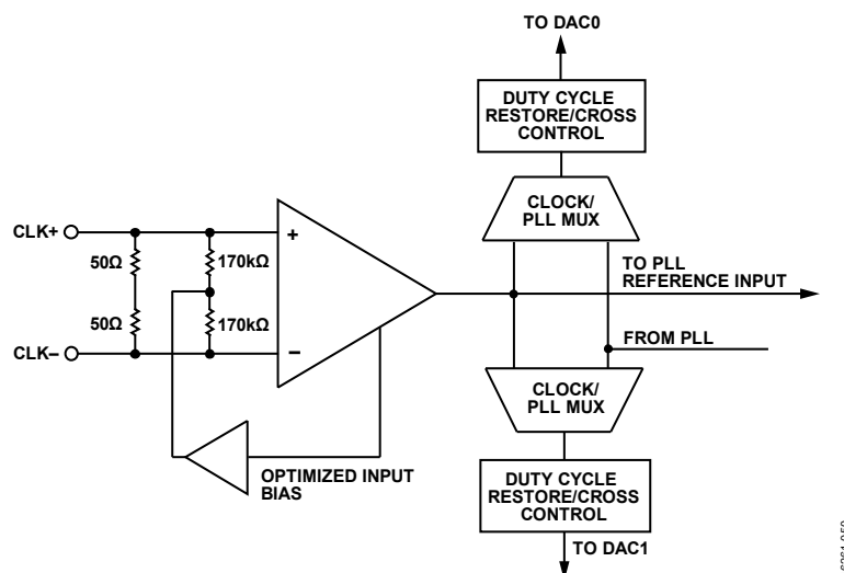
Figure 88. Clock Receiver Input Simplified Equivalent Circuit
