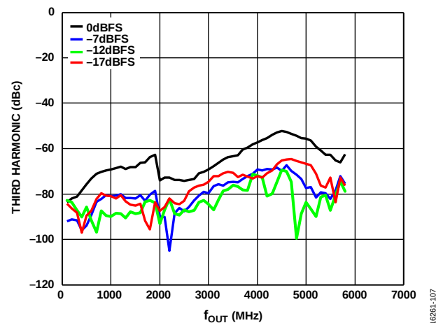
Figure 7. Third Harmonic (dBc) vs. f_{OUT} over Digital Scale (Mode 1), 12 GHz DAC Sample Rate, Channel Interpolation 4 \times , Main Interpolation 8 \times
