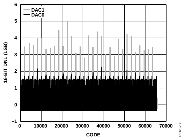
Figure 35. DNL, I_{OUTS} = 26\text{ mA} , 16-Bit Resolution
