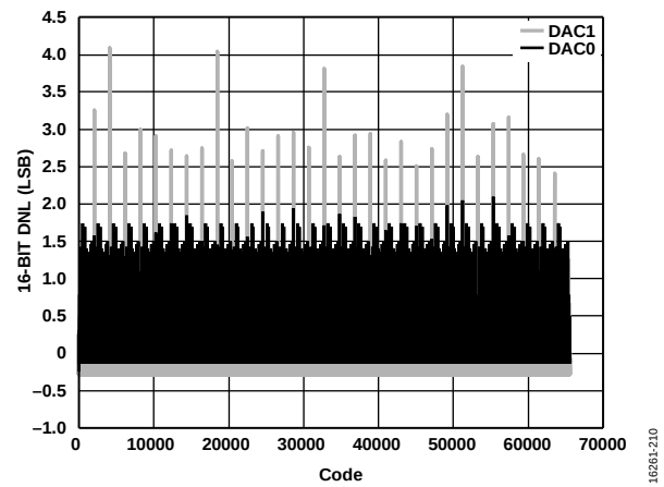
Figure 37. DNL, I_{OUTS} = 20\text{ mA} , 16-Bit Resolution
