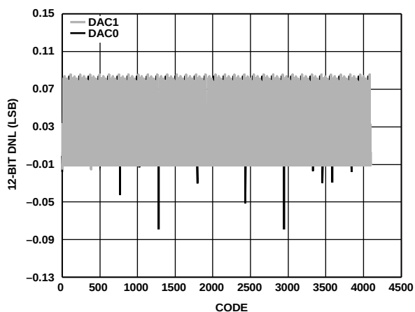
Figure 41. DNL, I_{OUTFS} = 20 mA, 12-Bit Resolution
