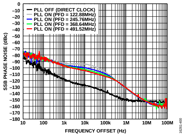
Figure 33. Single-Sideband (SSB) Phase Noise vs. Frequency Offset, over PFD Frequency, f_{DAC} = 12\text{ GHz} , f_{OUT} = 1.8\text{ GHz}
