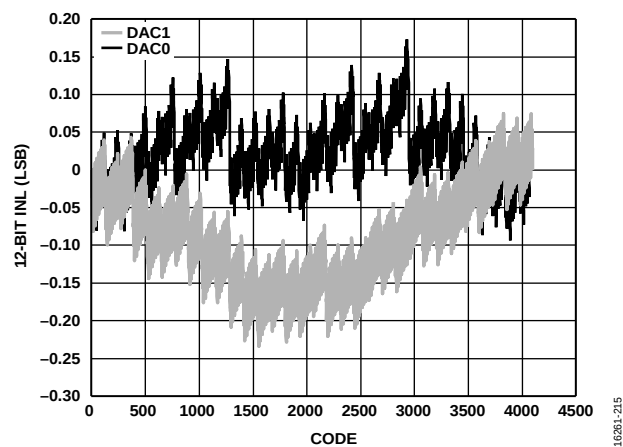
Figure 42. INL, I_{OUTFS} = 20 mA, 12-Bit Resolution
