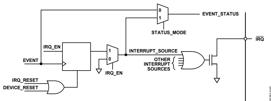
Figure 83. Simplified Schematic of \overline{\text{IRQx}} Circuitry
