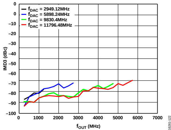
Figure 22. IMD3 vs. f_{OUT} over f_{DAC} (Mode 2), Channel Interpolation 4 \times , Main Interpolation 8 \times , 1 MHz Tone Spacing
