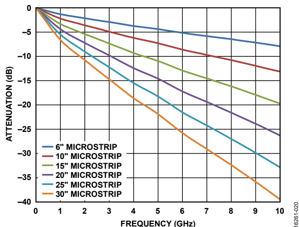
Figure 56. Insertion Loss of 50 \Omega Microstrips on FR4
