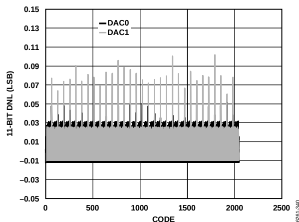
Figure 43. DNL, I_{OUTFS} = 20 mA, 11-Bit Resolution
