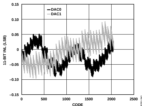
Figure 44. INL, I_{OUTFS} = 20 mA, 11-Bit Resolution
