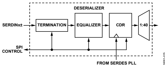
Figure 51. Deserializer Block Diagram
