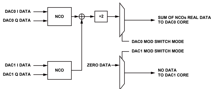
Figure 82. Mode 3—DAC0 = I0 + I1, DAC1 = 0
