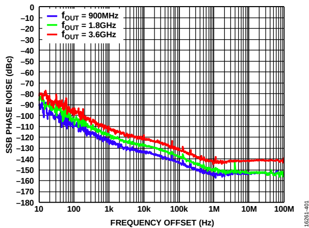
Figure 34. SSB Phase Noise vs. Frequency Offset over f_{OUT} , f_{DAC} = 12\text{ GHz} , Direct Clock (PLL Off)
