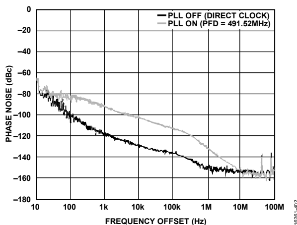
Figure 89. Phase Noise vs. Frequency Offset; Direct Clock and PLL Phase Noise, 12 GHz DAC Sample Rate, 1.65 GHz Output Frequency
