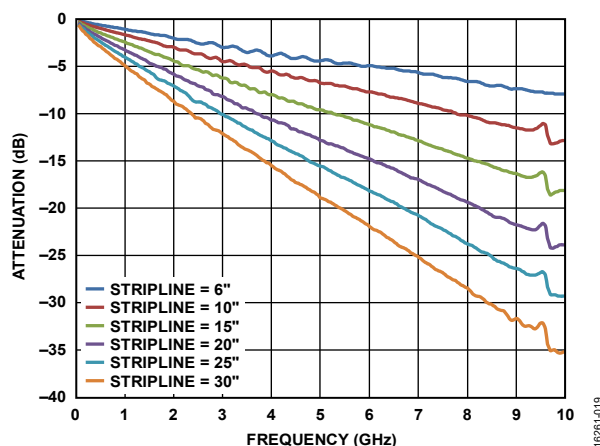
Figure 55. Insertion Loss of 50 \Omega Striplines on FR4
