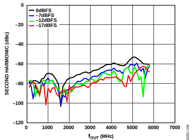
Figure 6. Second Harmonic (dBc) vs. f_{OUT} over Digital Scale (Mode 1), 12 GHz DAC Sample Rate, Channel Interpolation 4 \times , Main Interpolation 8 \times
