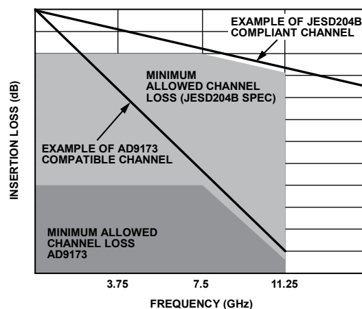
Figure 54. Insertion Loss Allowed
