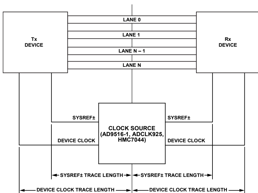
Figure 87. SYSREF \pm Signal and Device Clock Trace Length
