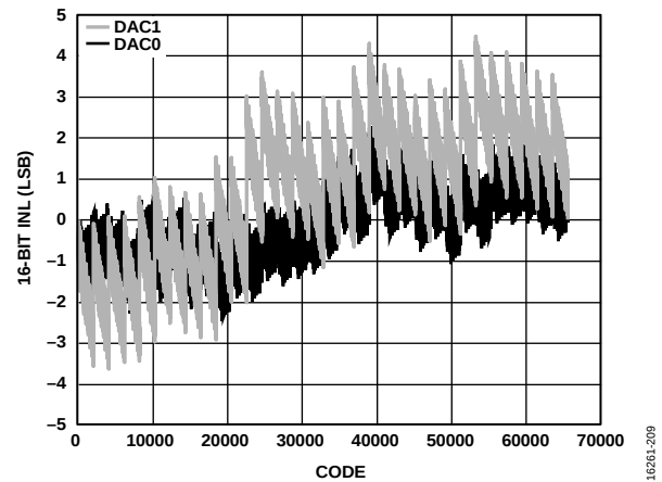
Figure 36. INL, I_{OUTS} = 26\text{ mA} , 16-Bit Resolution
