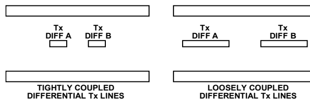
Figure 86. Tightly Coupled vs. Loosely Coupled Differential Traces
