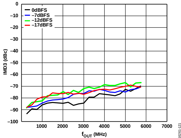
Figure 21. IMD3 vs. f_{OUT} over Digital Scale (Mode 2), 12 GHz DAC Sample Rate, Channel Interpolation 4 \times , Main Interpolation 8 \times , 1 MHz Tone Spacing
