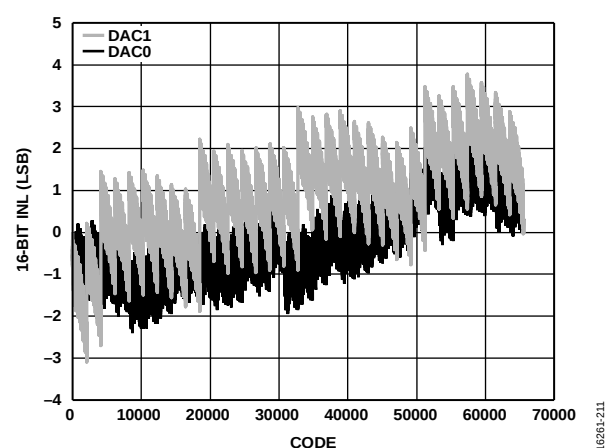
Figure 38. INL, I_{OUTS} = 20\text{ mA} , 16-Bit Resolution
