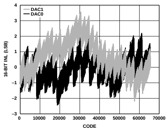
Figure 40. INL, I_{OUTFS} = 15.6 mA, 16-Bit Resolution
