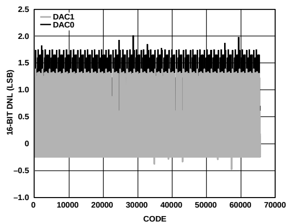
Figure 39. DNL, I_{OUTFS} = 15.6 mA, 16-Bit Resolution
