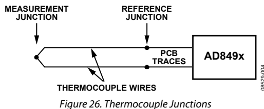
Figure 26. Thermocouple Junctions
