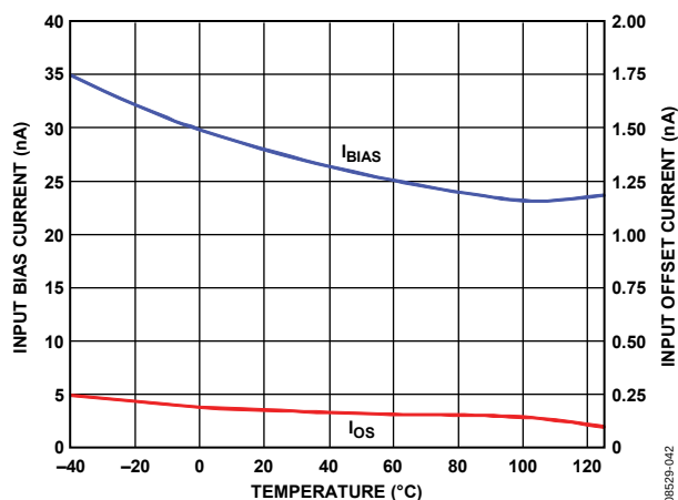
Figure 8. Input Bias Current and Input Offset Current vs. Temperature
