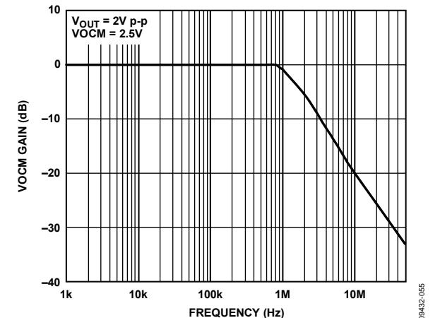
Figure 28. VCM Large Signal Frequency Response
