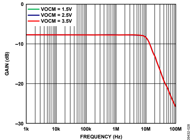
Figure 27. Large Signal Frequency Response for Various VCM Levels
