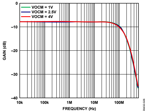
Figure 24. Small Signal Frequency Response for Various VCM Levels
