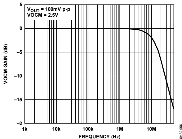
Figure 25. VCM Small Signal Frequency Response
