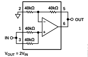
Figure 46. Noninverting Amplifier, Gain = 2
