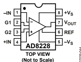
Figure 44. Pinout Diagram
