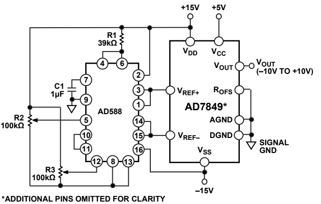
Figure 21. Bipolar \pm 10 \text{ V} Operation
