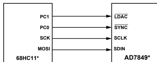
Figure 26. AD7849-to-68HC11 Interface
