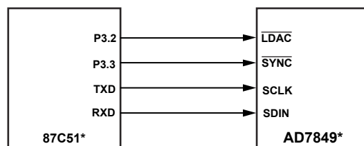
Figure 27. AD7849-to-87C51 Interface
