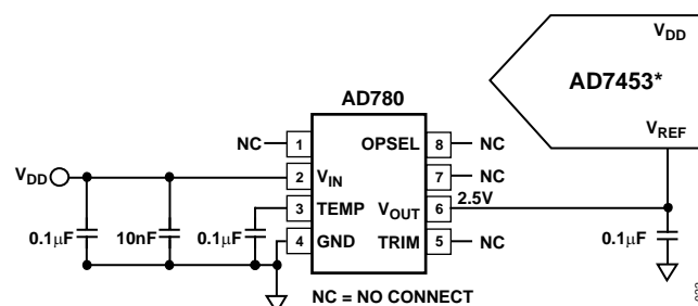
Figure 22. Typical V_{REF} Connection Diagram for V_{DD} = 5\text{ V}
