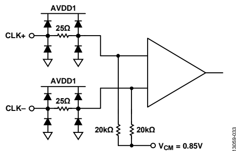
Figure 34. Clock Inputs
