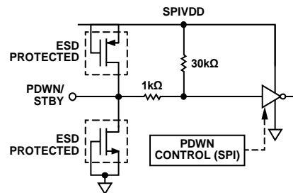
Figure 41. PDWN/STBY Input
