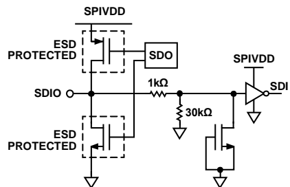
Figure 39. SDIO
