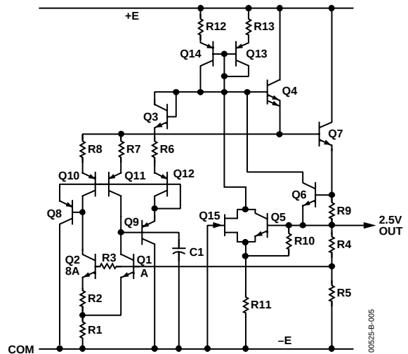
Figure 5. Schematic Diagram
