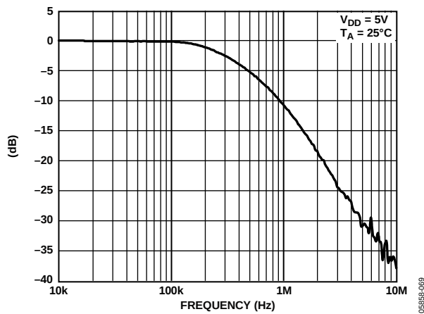
Figure 47. Multiplying Bandwidth
