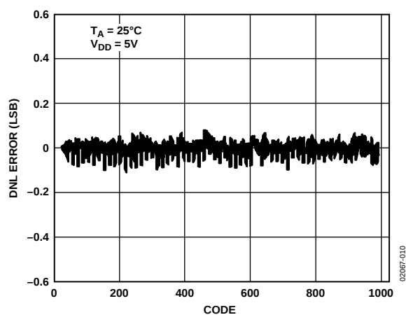
Figure 10. AD5317 DNL
