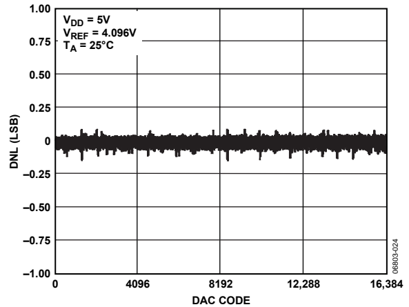
Figure 13. AD5024 DNL
