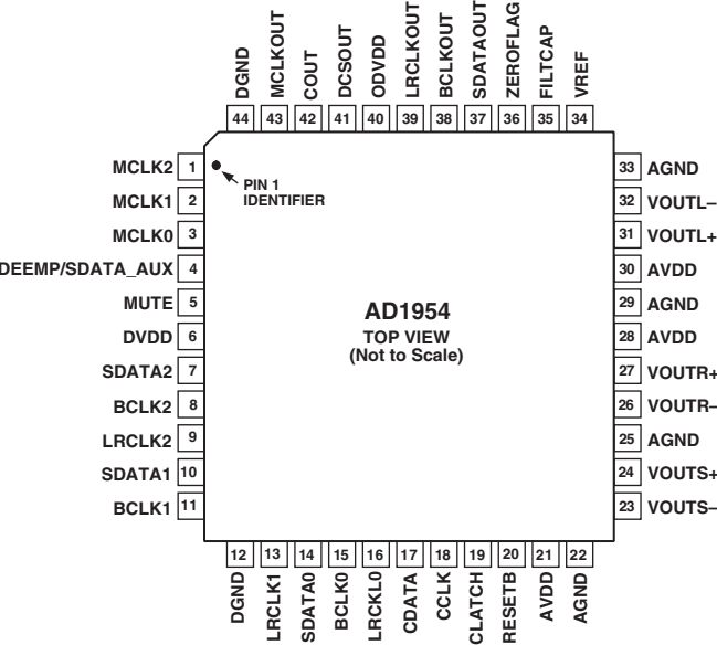
44-LEAD MQFP
