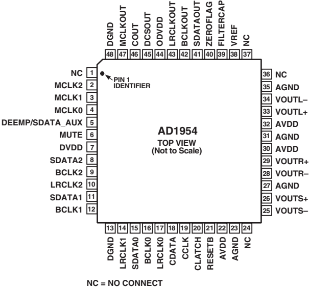
48-LEAD LQFP
