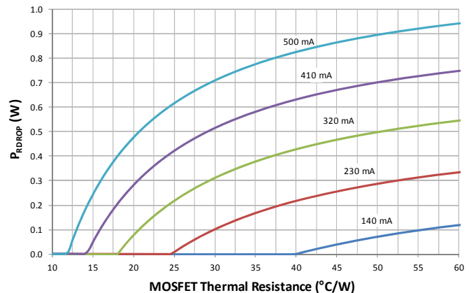
Figure 9. R_{DROD} Dissipation versus MOSFET thermal resistance at various V33 regulator maximum current settings, I_{V33ILIM}
