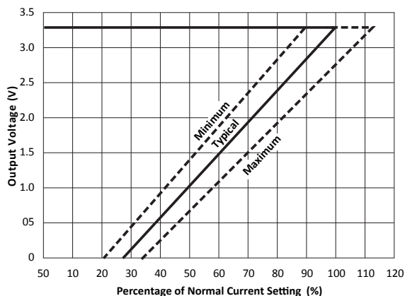
Figure 7. Foldback current limit of the V33 regulator
