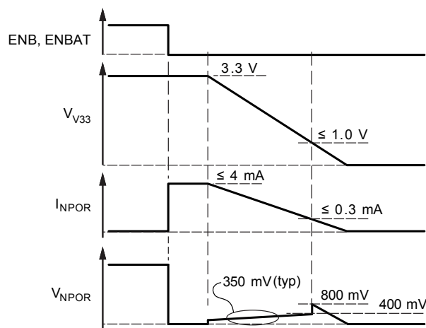
Figure 3. NPOR and V33 characteristics when the A4406 is disabled
