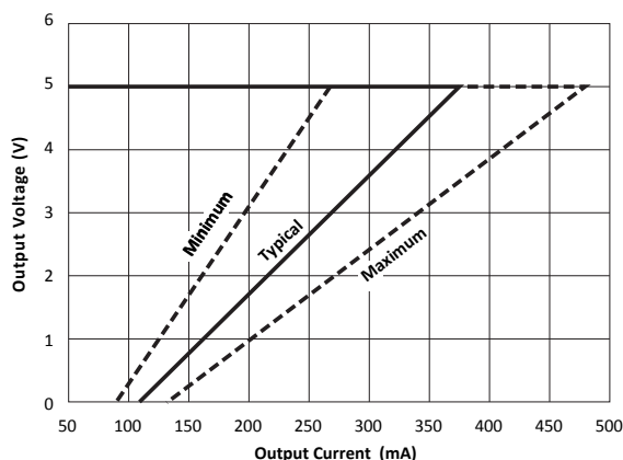
Figure 4. Foldback current limit of the 5VP regulator
