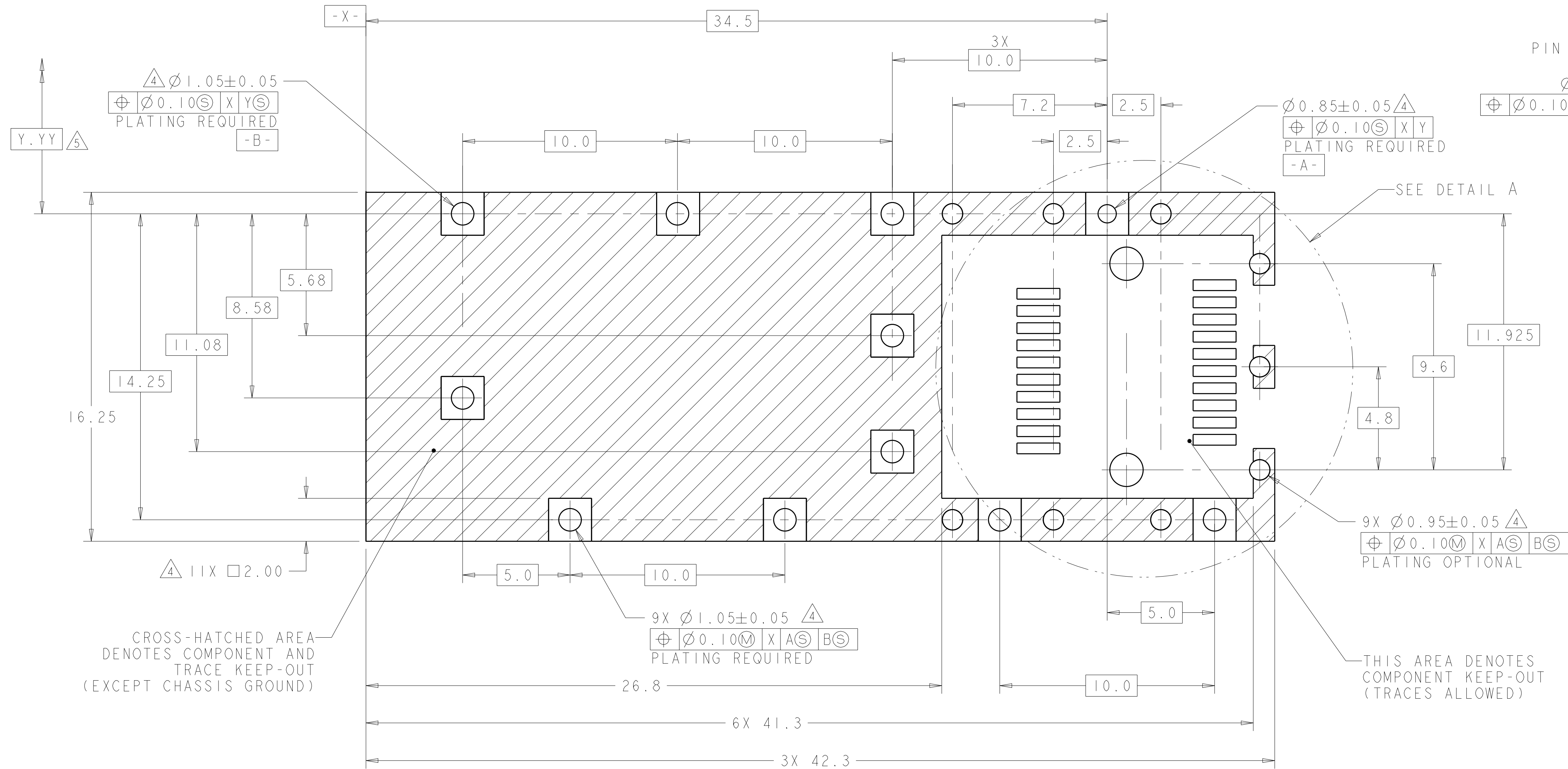
2110304-1/-5/-6/-7 RECOMMENDED PCB LAYOUT SCALE 8:1
