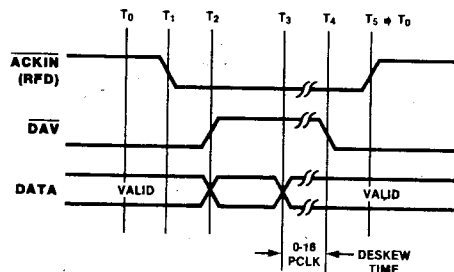
Figure 3-10. Strobed Output Handshake Timing Diagram
