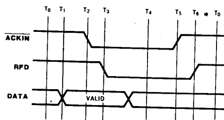
Figure 3-3. Interlocked Input Handshake Timing Diagram
