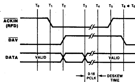
Figure 3-9. Interlocked Output Handshake Timing Diagram
