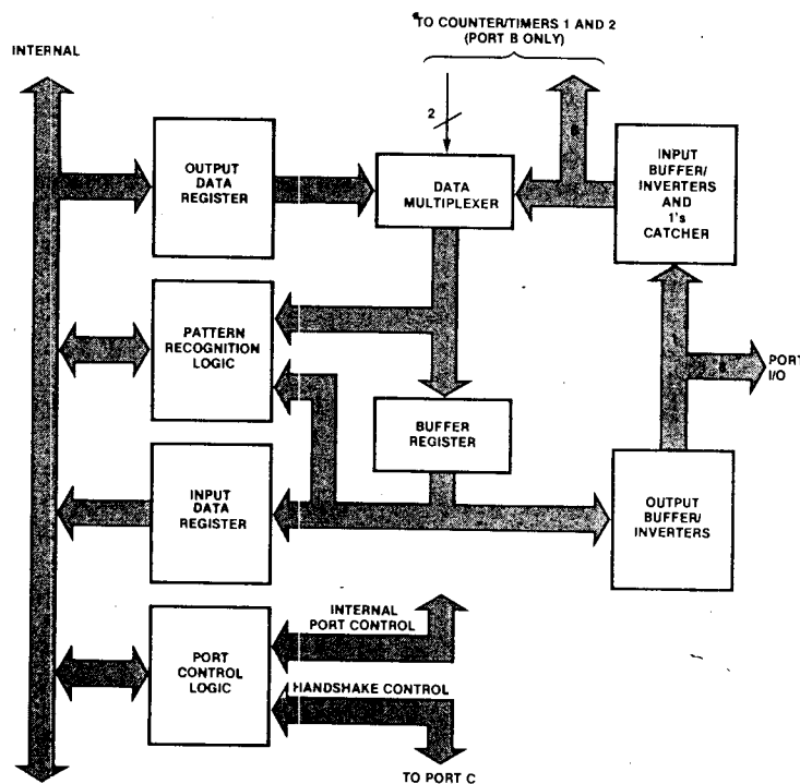
Figure 1-2. Ports A and B Block Diagram
