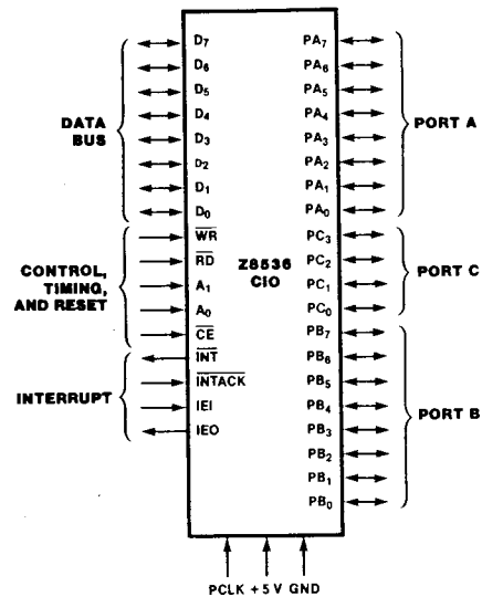
Figure 8-1. Z8536 (CIO) Pin Functions
