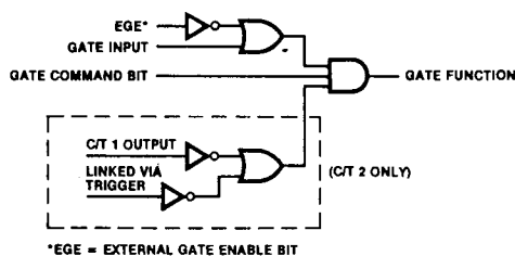
Figure 4-3. Gate AND-Function Diagram
