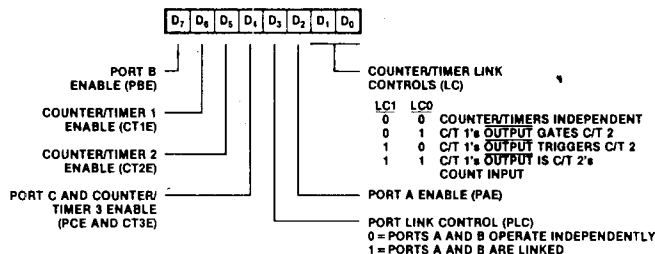
Figure 2-3. Master Configuration Control Register
