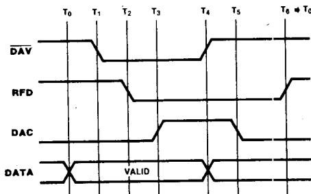
Figure 3-7. 3-Wire Input Handshake Timing Diagram
