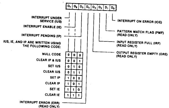
Figure 2-6. Port Command and Status Registers
