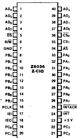
Figure 7-2. Z8036 (Z-CIO) Pin Assignments
