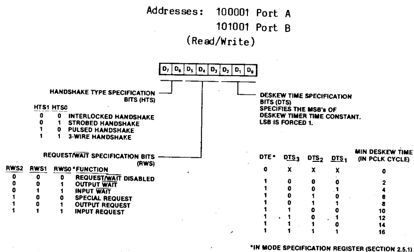
Figure 2-5. Port Handshake Specification Registers
