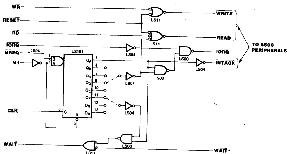
Figure 5-4. \overline{\text{WAIT}} and \overline{\text{INTACK}} Generation Logic
