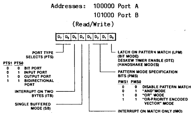
Figure 2-4. Port Mode Specification Registers
