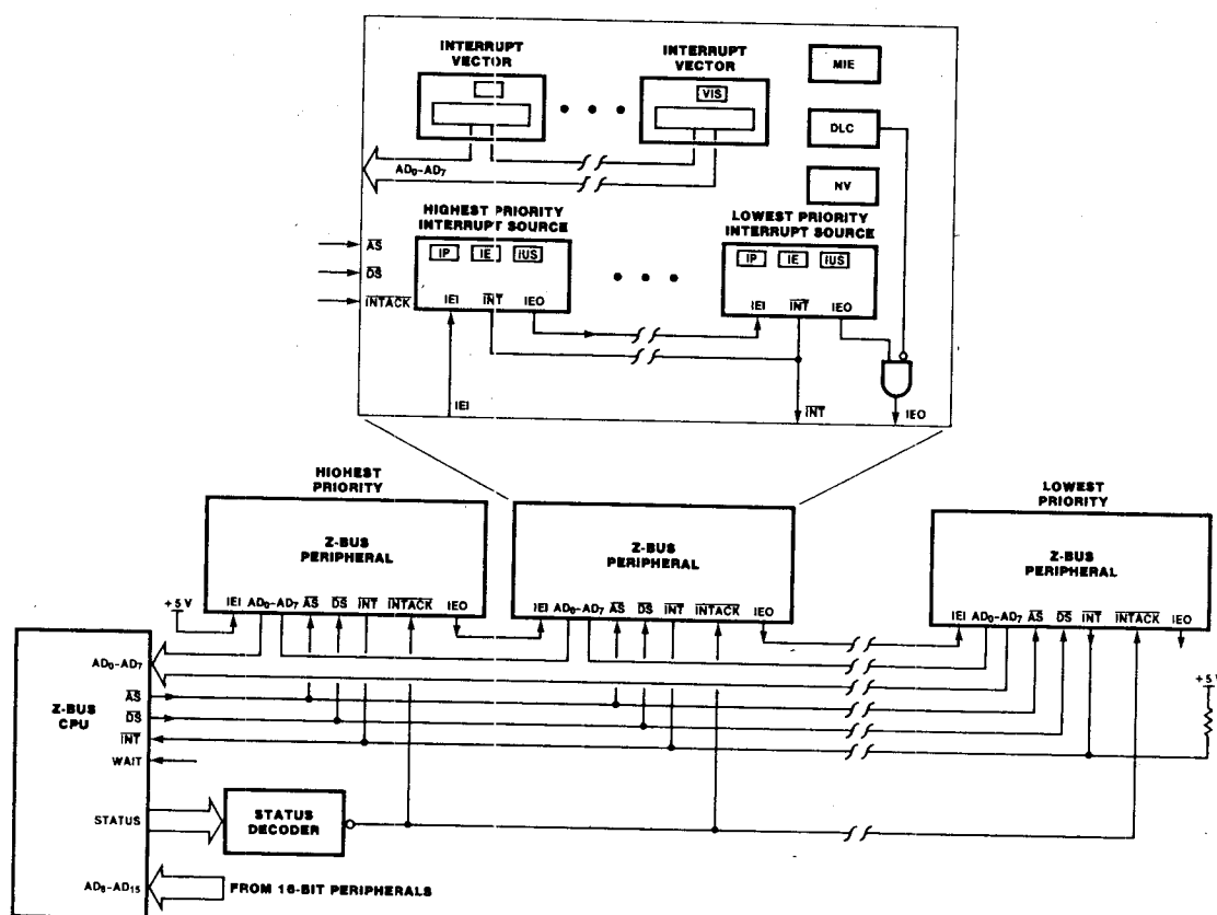
Figure 5-2. Z-BUS Interrupt Arbitration
