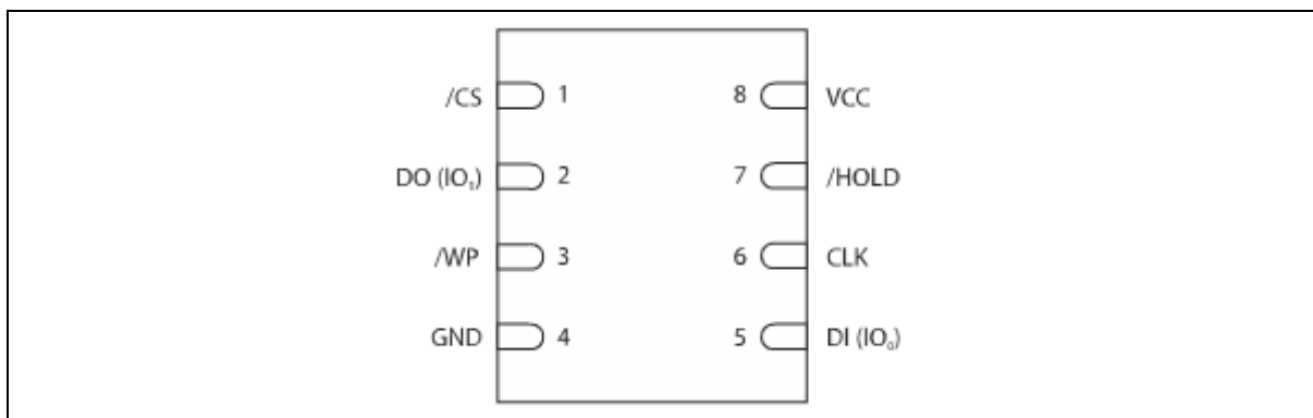
Figure 1b. W25X10CL Pad Assignments, 8-pad WSON 6x5-MM and USON 2x3-MM (Package Code ZP & UX)
