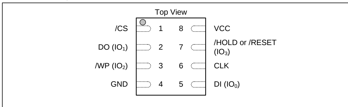
Figure 1a. W25Q512JV Pad Assignments, 8-pad WSON 8x6-mm (Package Code E)
