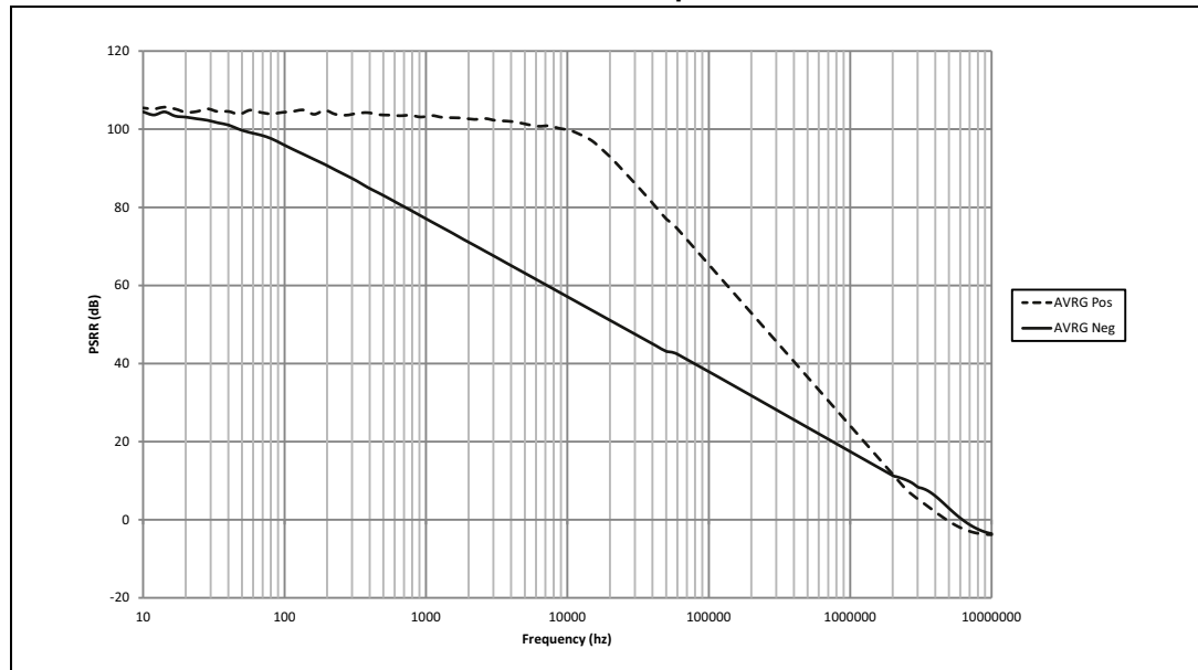
Figure 13. PSRR for TS924/TS924A at V_{CC} = 5\text{ V} , V_{icm} = 2.5\text{ V} , T = 25\text{ }^{\circ}\text{C} , R_I = 100\text{ k}\Omega , and C_I = 100\text{ pF}
