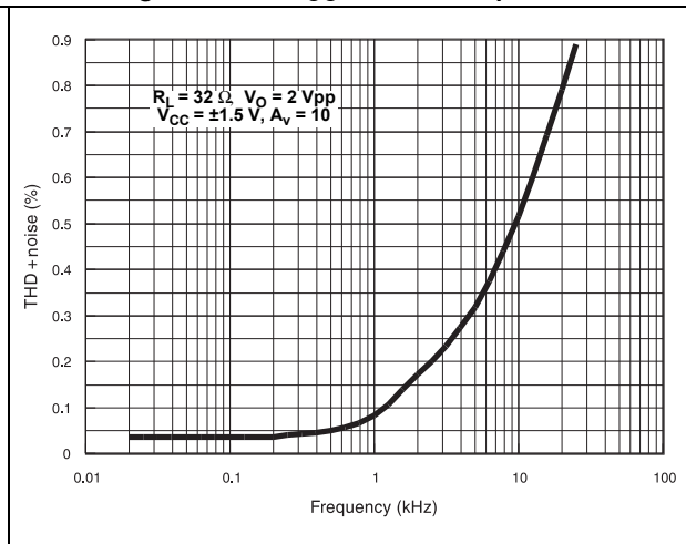
Figure 8. THD + noise vs. frequency ( R_L = 32\text{ }\Omega , V_O = 2\text{ Vpp} , V_{CC} = \pm 1.5\text{ V} , A_V = 10 )
