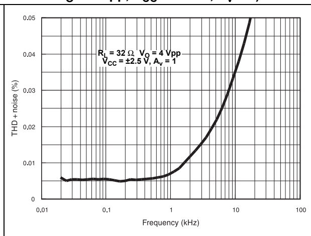
Figure 10. THD + noise vs. frequency ( R_L = 32\text{ }\Omega , V_O = 4\text{ Vpp} , V_{CC} = \pm 2.5\text{ V} , A_V = 1 )
