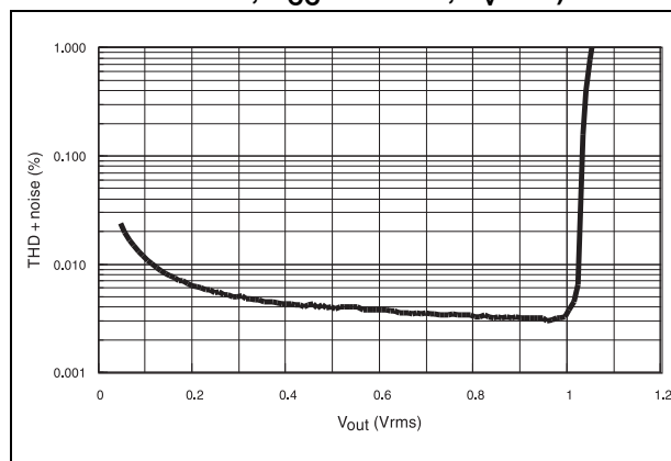
Figure 11. THD + noise vs. V_{out} ( R_L = 600\text{ }\Omega , f = 1\text{ kHz} , V_{CC} = \pm 1.5\text{ V} , A_V = -1 )
