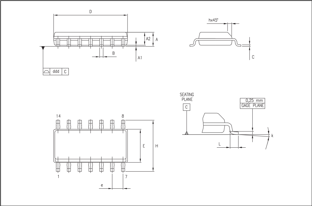
Figure 14. SO14 package outline
