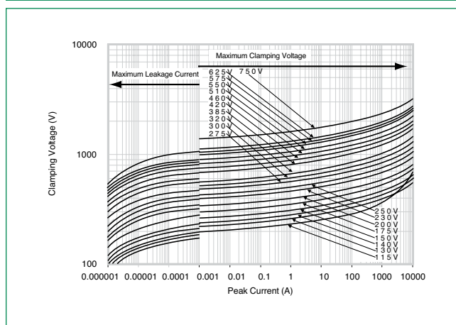
Figure 4. Maximum Clamping Voltage for 20mm Parts
