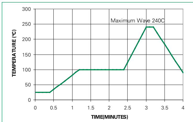
Figure 7. Non Lead-free Profile
