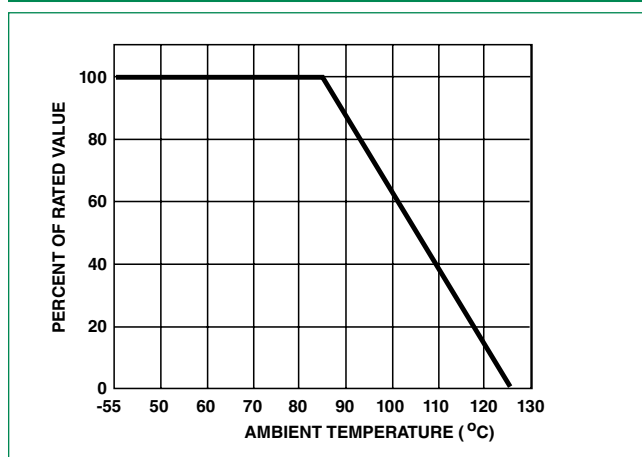
Figure 2. Current, Energy, Power Derating Curve
