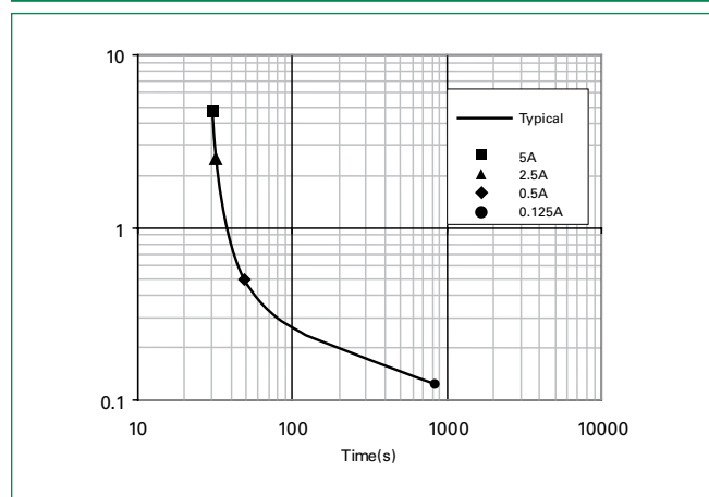
Figure 1. Thermal Characteristics
