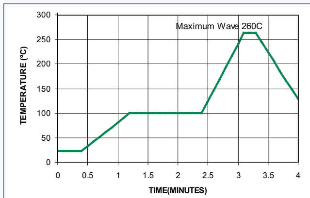
Figure 8. Lead-free Profile
