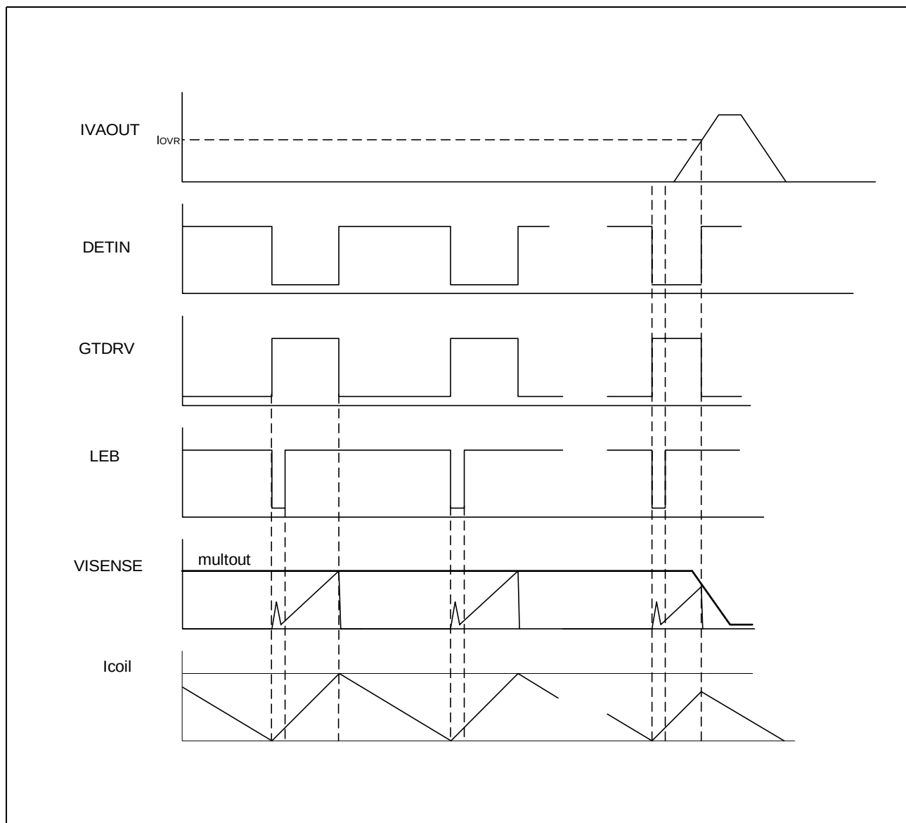
Figure 4 Typical signals
