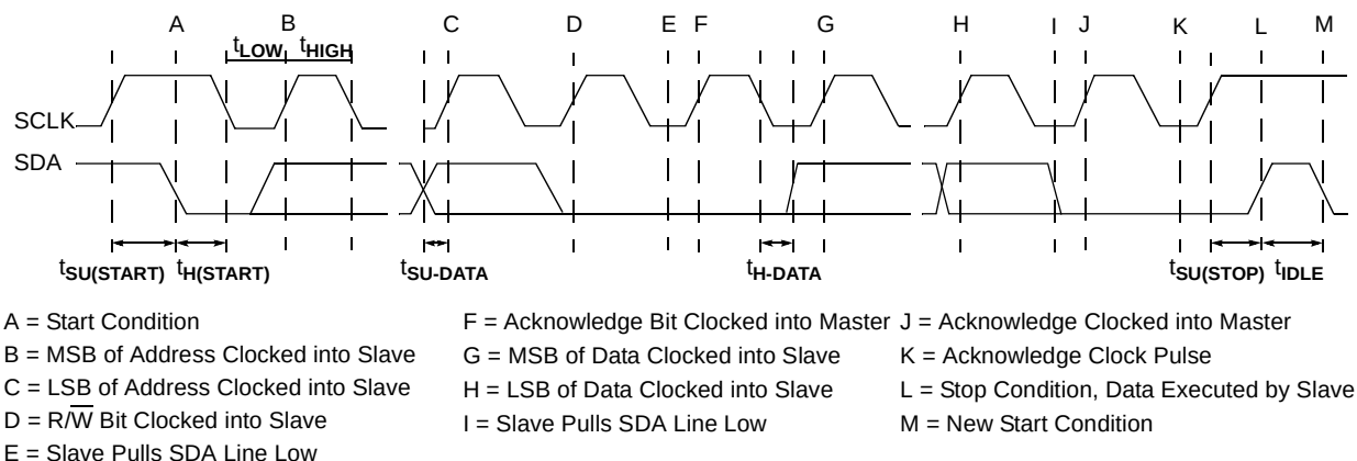
FIGURE 1-1: Timing Diagrams.
