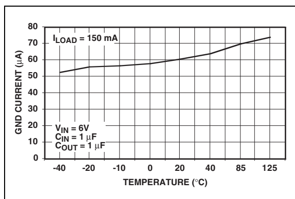
FIGURE 2-15: GND Current vs. Temperature ( I_{I_{OAD}} = 150 \text{ mA} ).
