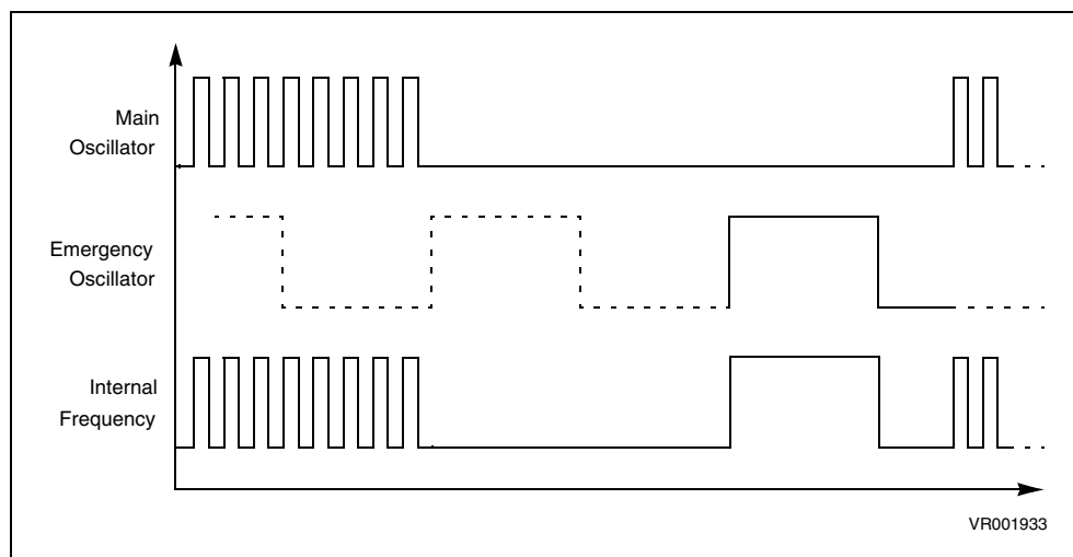
Figure 11. OSG Emergency Oscillator Principle
