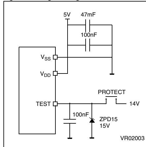
Figure 55. Programming Circuit
