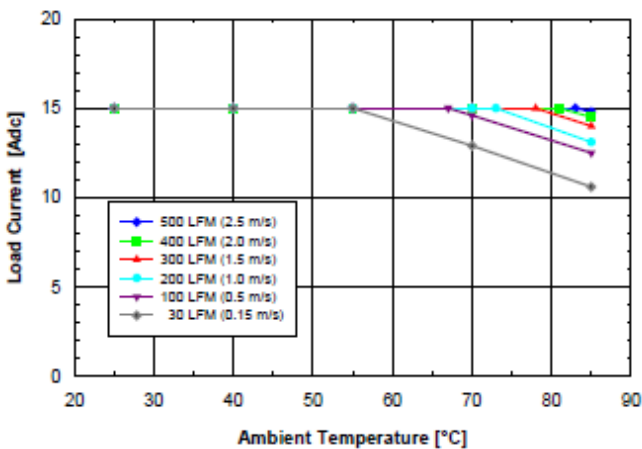
Fig. 2.5V.2: Available load current vs. ambient air temperature and airflow rates for SQ48T15025 converter with D height pins mounted horizontally with Vin = 48 V, air flowing from pin 3 to pin 1, and maximum FET temperature ≤ 120 °C.
