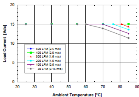
Fig. 2.0V.1: Available load current vs. ambient temperature and airflow rates for SQ48T15020 converter with D height pins mounted vertically with V_{in} = 48\text{ V} , air flowing from pin 3 to pin 1, and maximum FET temperature \leq 120^\circ\text{C} .
