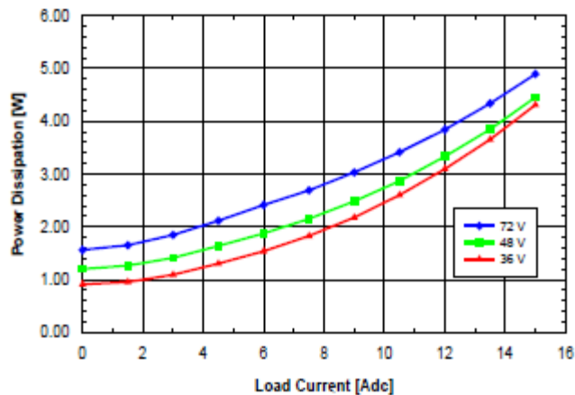
Fig. 1.8V.7: Power dissipation vs. load current and input voltage for SQ48T/S15018 converter mounted vertically with air flowing from pin 3 to pin 1 at a rate of 300 LFM (1.5 m/s) and T_a = 25^\circ\text{C} .
