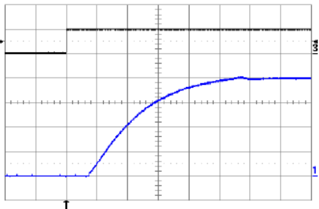
Fig. 8.0V.10: Turn-on transient at full rated load current (resistive) plus 2,200 \mu\text{F} at V_{in} = 48\text{V} , triggered via ON/OFF pin. Top trace: ON/OFF signal (5 V/div.). Bottom trace: output voltage (2 V/div.). Time scale: 2 ms/div.
