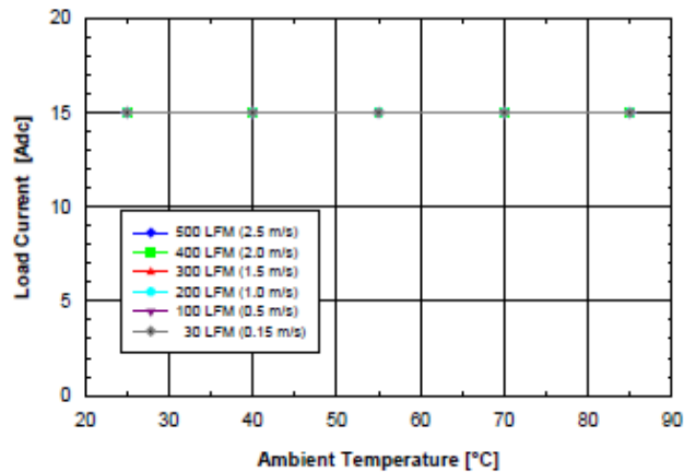
Fig. 1.0V.4: Available load current vs. ambient air temperature and airflow rates for SQ48S15010 converter mounted horizontally with V_{in} = 48\text{ V} , air flowing from pin 3 to pin 1, and maximum FET temperature \leq 120\text{ }^{\circ}\text{C} .
