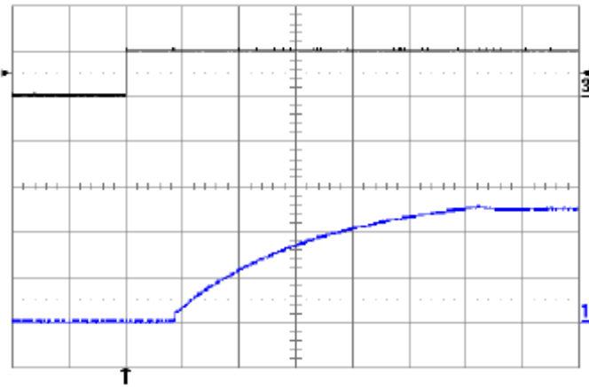
Fig. 5.0V.10: Turn-on transient at full rated load current (resistive) plus 10,000 \mu F at V_{in} = 48V , triggered via ON/OFF pin. Top trace: ON/OFF signal (5 V/div.). Bottom trace: output voltage (2 V/div.). Time scale: 2ms/div.
