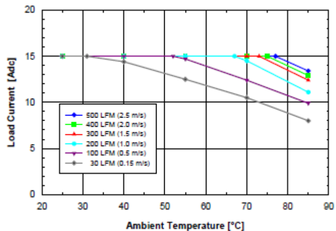
Fig. 3.3V.1: Available load current vs. ambient air temperature and airflow rates for SQ48T15033 converter with D height pins mounted horizontally with Vin = 48V, air flowing from pin 3 to pin 1, and maximum FET temperature ≤ 120°C.
