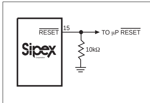
Figure 18. External Pull-down Resistor Ensures \overline{\text{RESET}} is Valid with V_{\text{CC}} Down to Ground.
