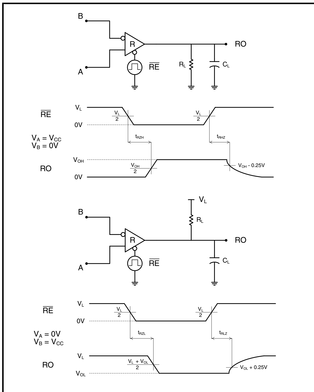
FIGURE 12. RS-485/422 RECEIVER OUTPUT ENABLE/DISABLE TIMES
