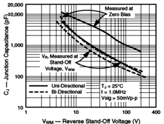
Figure 4. Typical Junction Capacitance Uni-Directional
