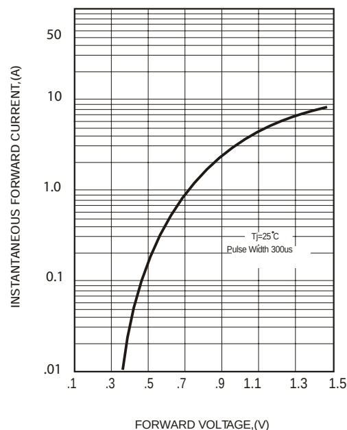
FIG.7-TYPICAL FORWARD CHARACTERISTICS
