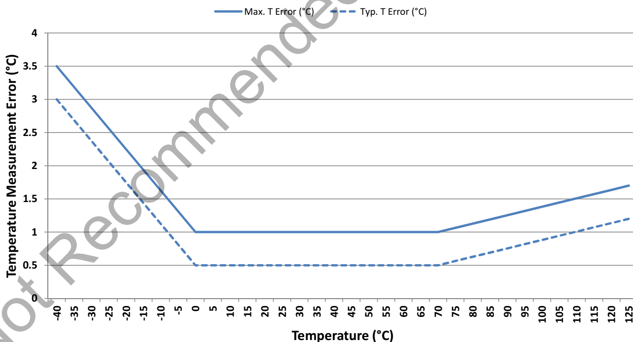
Figure 3. Temperature Accuracy
