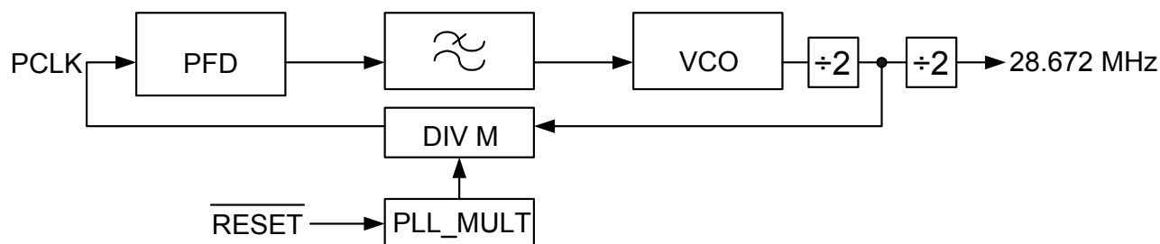
Figure 40. PLL Frequency Synthesizer
