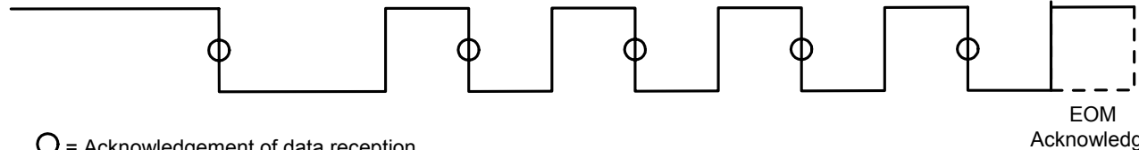
Figure 61. Example Write to Registers $10 and $11 in Channel 0 of the Dual ProSLIC
