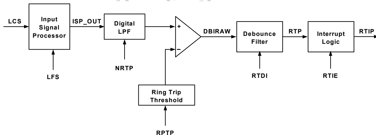
Figure 23. Ring Trip Detector
