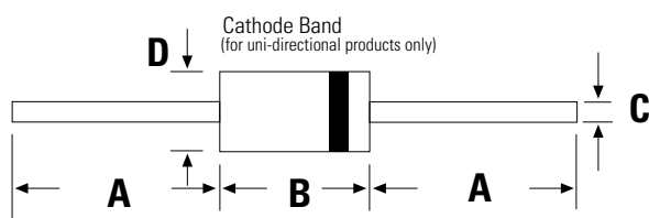
DO-204AC (DO-15)
