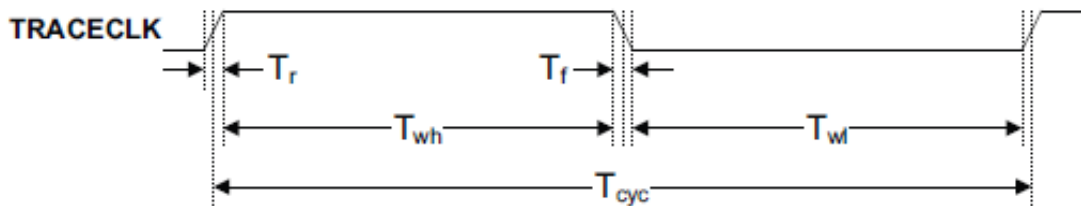
Figure 11. TRACE_CLKOUT specifications
