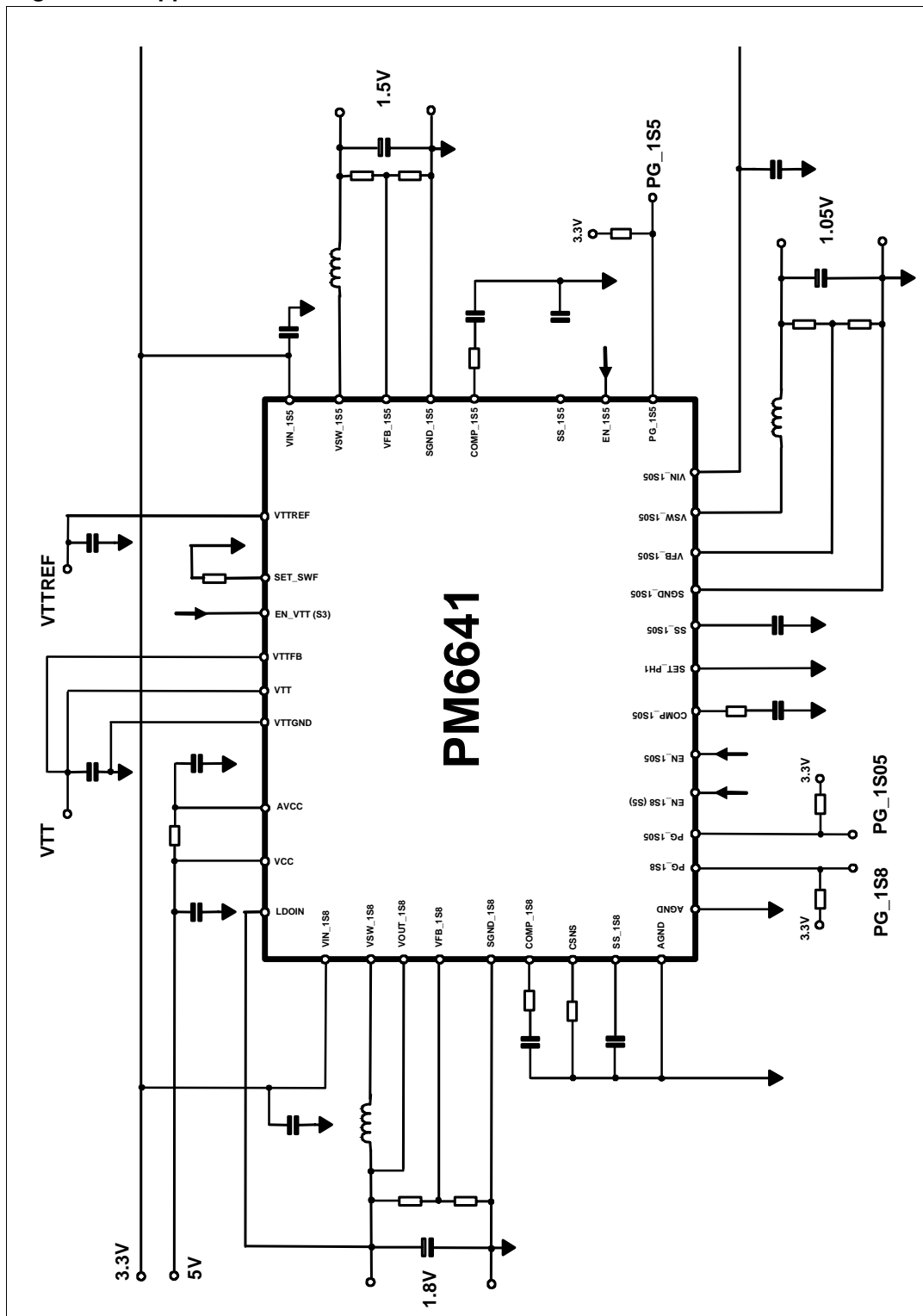
Figure 1. Application circuit
