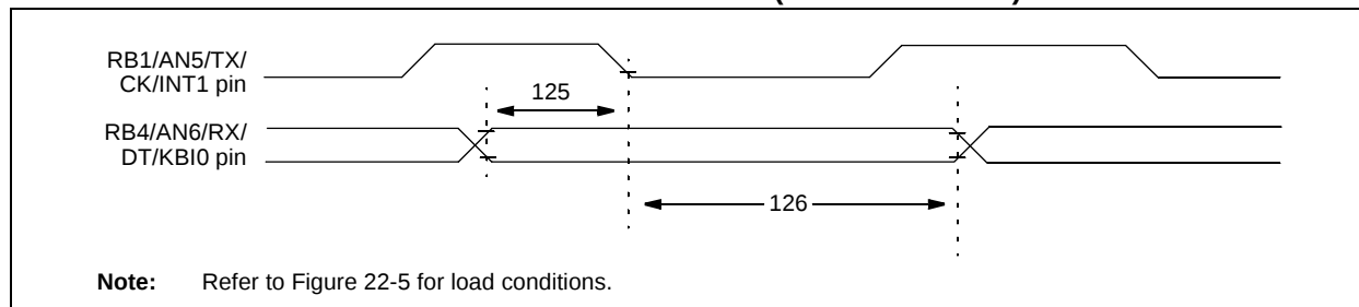
FIGURE 22-13: EUSART SYNCHRONOUS RECEIVE (MASTER/S�AVE) TIMING
