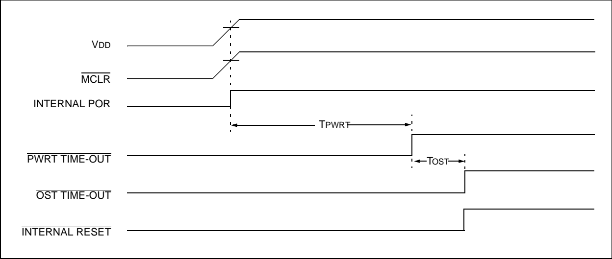
FIGURE 8-12: TIME-OUT SEQUENCE ON POWER-UP ( \overline{\text{MCLR}} TIED TO \text{V}_{\text{DD}} ): FAST \text{V}_{\text{DD}} RISE TIME
