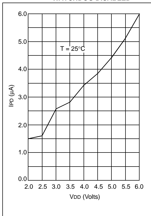
FIGURE 13-5: TYPICAL I_{PD} vs. V_{DD} , WATCHDOG DISABLED
