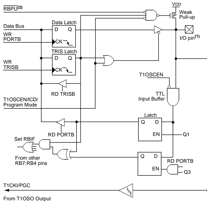
FIGURE 5-14: BLOCK DIAGRAM OF RB6 PIN
