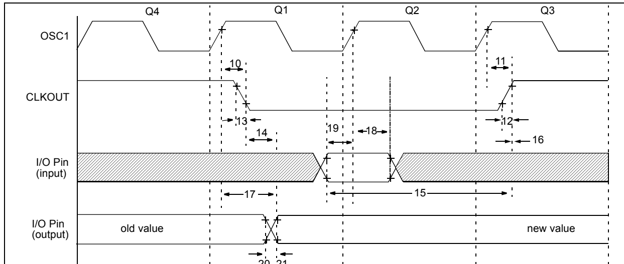
FIGURE 12-5: CLKOUT AND I/O TIMING
