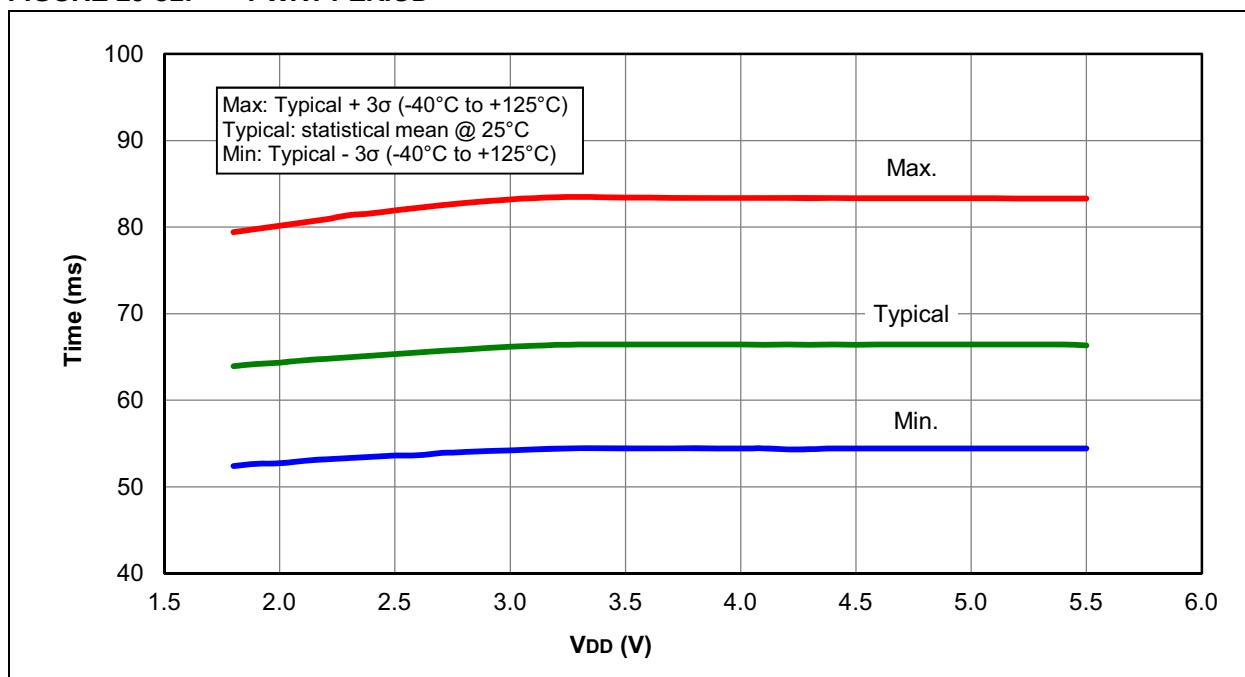
FIGURE 29-51: PWRT PERIOD
