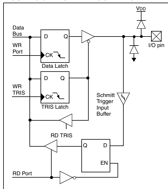
FIGURE 5-6: PORTD BLOCK DIAGRAM
