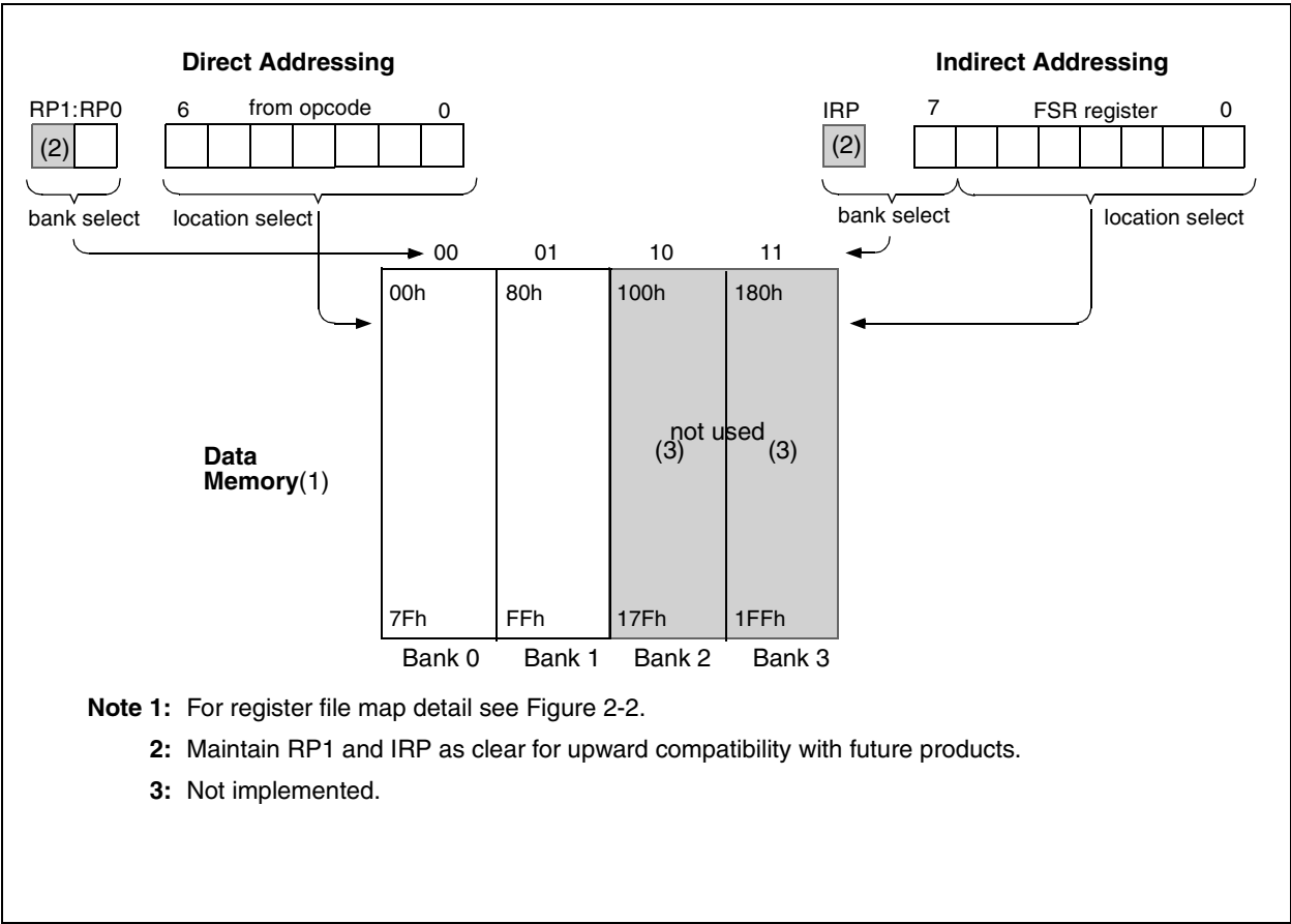
FIGURE 2-11: DIRECT/INDIRECT ADDRESSING
